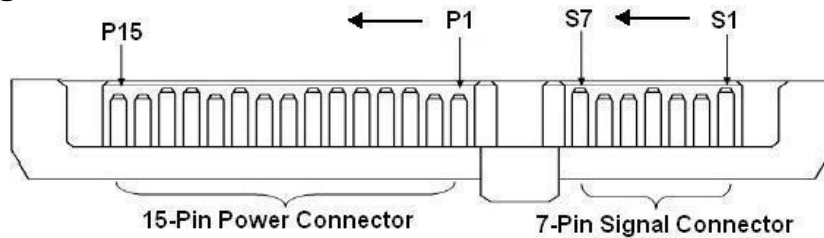
Figure 3 Pin connector
